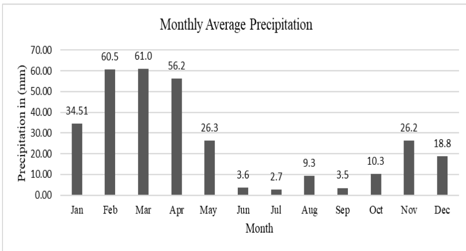
Figure 3: Monthly Average Precipitation from 2006-2020
